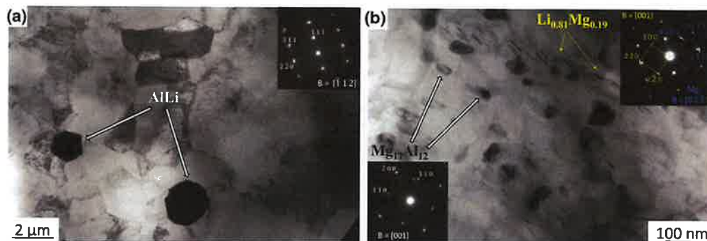
Fig. 4 TEM images in bright field and selected area diffraction (SAD) patterns obtained from second phase particles formed in Mg-4Li-3Al-1Zn: (a) extruded to Ø4 mm, (b) extruded to Ø1 mm
