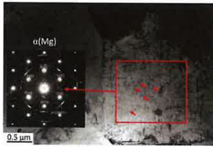
Fig. 8. TEM bright-field image of the WE43 KoBo extruded to Ø8 mm.
