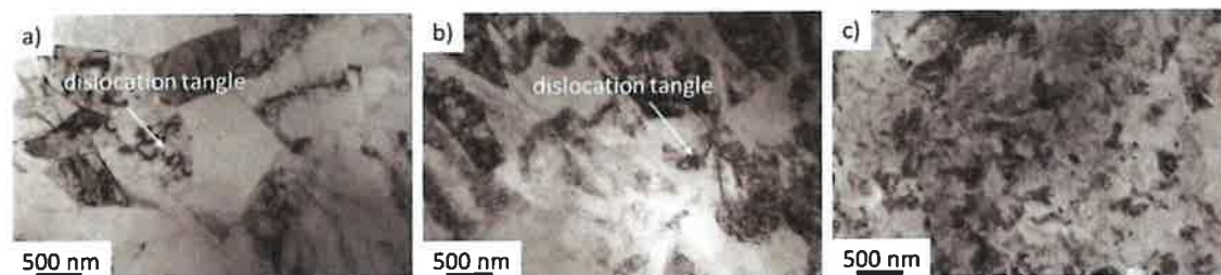
Fig. 5 – TEM micrographs of AZ31 extruded to (a) \varnothing 6 mm, (b) \varnothing 4 mm, and (c) \varnothing 2 mm.
