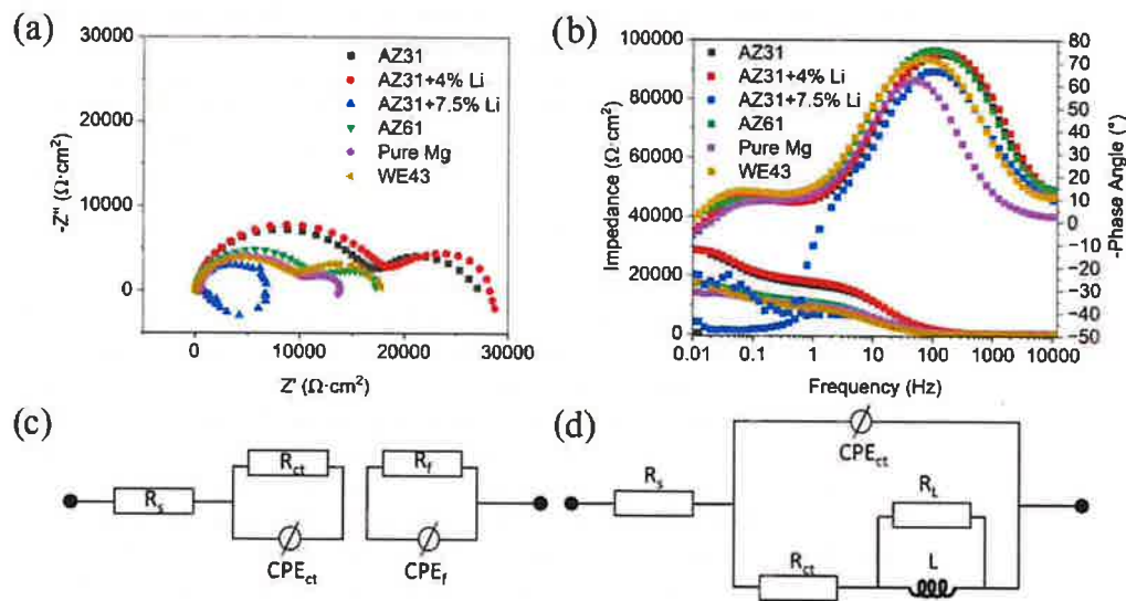
Figure 3. Electrochemical impedance spectroscopy (EIS) results recorded after 1 h of immersion in naturally aerated 0.1 M NaCl and presented in the form of (a) Nyquist plots, (b) Bode plots, (c) equivalent electrical circuit used for pure Mg, AZ31, AZ61, AZ31+4Li, and WE43 fitting, and (d) equivalent electrical circuit used for AZ31+7.5Li fitting.
