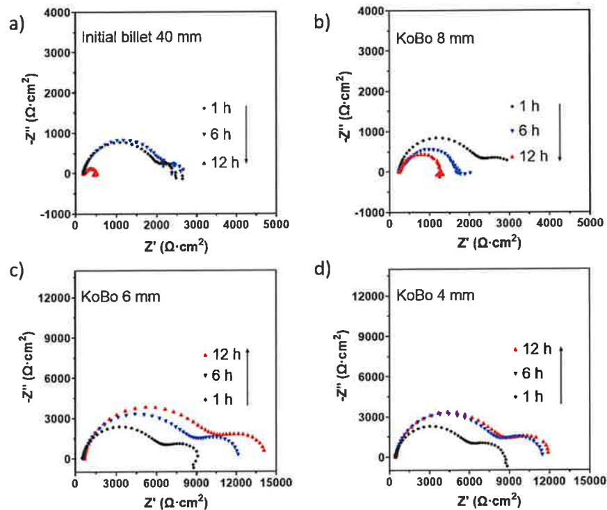
Figure 8. EIS results for pure Mg in naturally aerated 0.01 M NaCl delivered in the form of Nyquist plots: (a) initial billet, (b) KoBo-extruded to Ø8 mm, (c) KoBo-extruded to Ø6 mm, and (d) KoBo-extruded to Ø4 mm.
