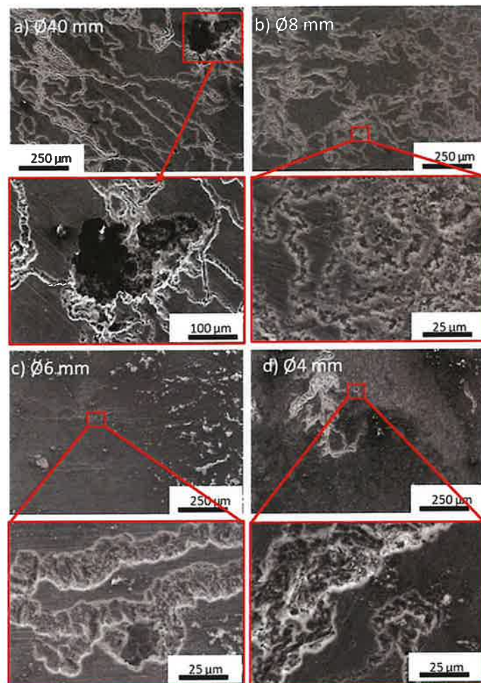
Figure 10. Corrosion damage observed on the surfaces of pure Mg after corrosion product removal after 1 h immersion in naturally aerated 0.01 M NaCl: (a) initial billet (Ø40 mm), (b) Ø8 mm, (c) Ø6 mm, and (d) Ø4 mm.
