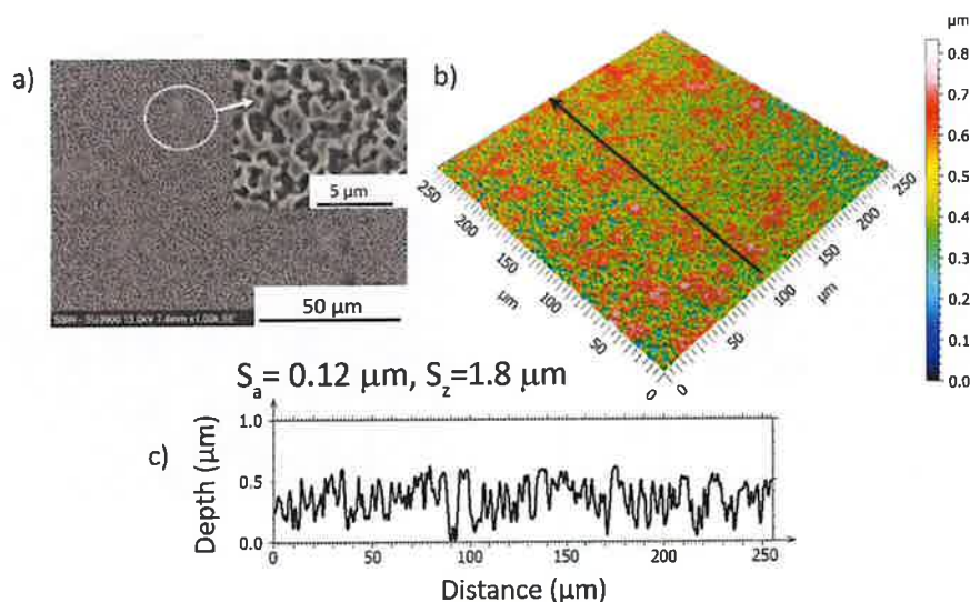
Fig. 13. Post-corrosion characterization of ED Cu: a) SEM image of the surface, b) CLSM 3D image, b) surface profile extracted from the location marked by the arrow.
