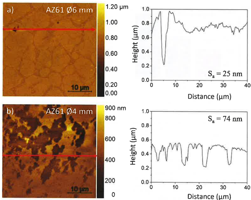
Fig. 14. AFM images with the corresponding surface development profiles extracted from the area marked by the arrow for a) AZ61 extruded to Ø6 mm, b) AZ61 extruded to Ø4 mm.
