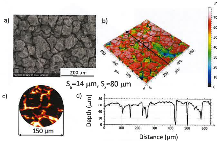
Fig. 14. Post-corrosion characterization of CS Cu: a) SEM image, b) 3D CLSM image, c) D-SIMS elemental map for ^{16}\text{O} , d) surface profile extracted from the area marked by the arrow in panel b.
