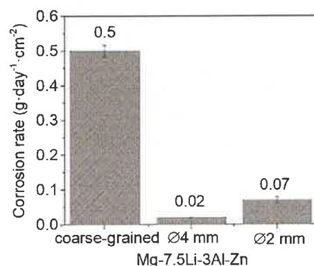
Fig. 8. Corrosion rate calculated after 1 h of immersion in 0.1 M NaCl for conventionally extruded and annealed Mg-7.5Li-3Al-1Zn (coarse-grained), and for Mg-7.5Li-3Al-1Zn KoBo extruded to Ø4 mm and Ø2 mm.
