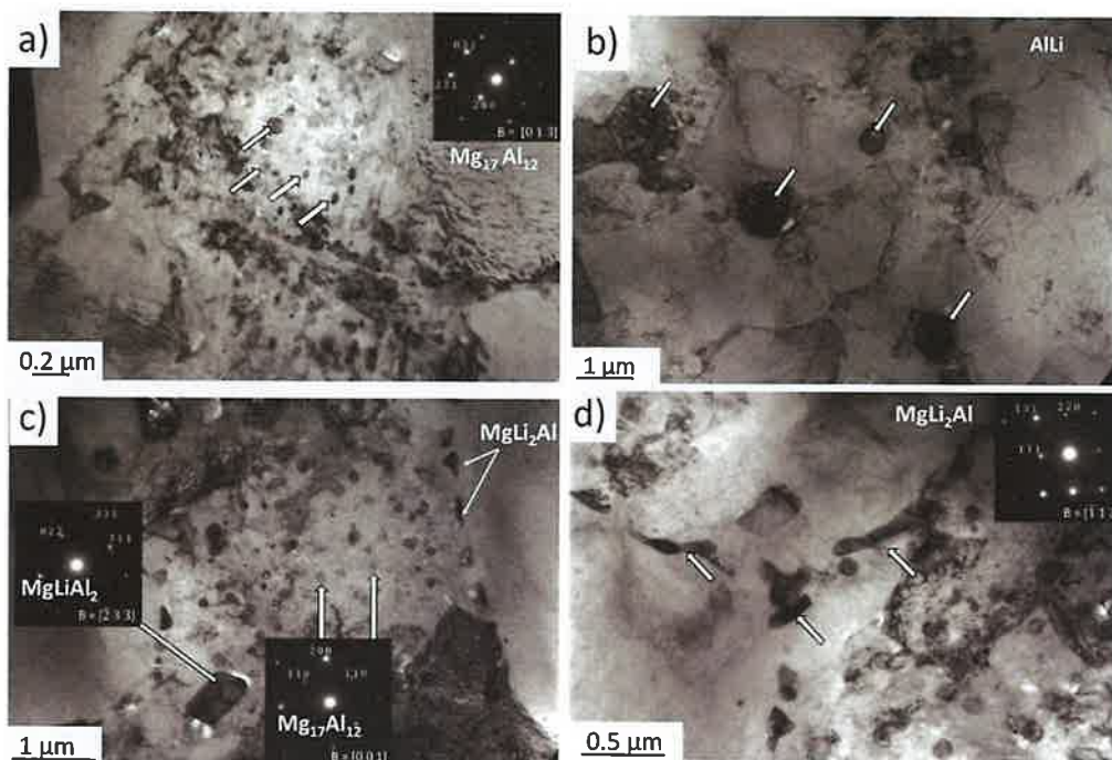
Fig. 4. TEM images in bright field and selected area diffraction (SAD) patterns obtained from the alloy extruded to Ø4 mm (a and b), and the alloy extruded to Ø2 mm (c and d).
