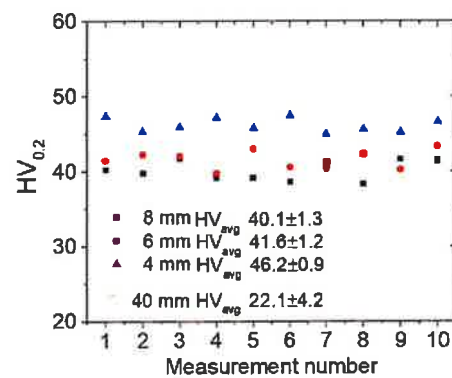
Figure 6. Microhardness profiles of the pure Mg initial billet and pure Mg KoBo-extruded to Ø8 mm, Ø6 mm, or Ø4 mm.
