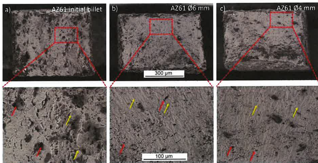
Fig. 9. Fracture surfaces of the AZ61 alloys: a) initial billet, b) KoBo extruded to Ø6 mm and c) KoBo extruded to Ø4 mm. Dimples are marked by the red arrows, and facets typical for brittle fracture are marked by the yellow arrows.
