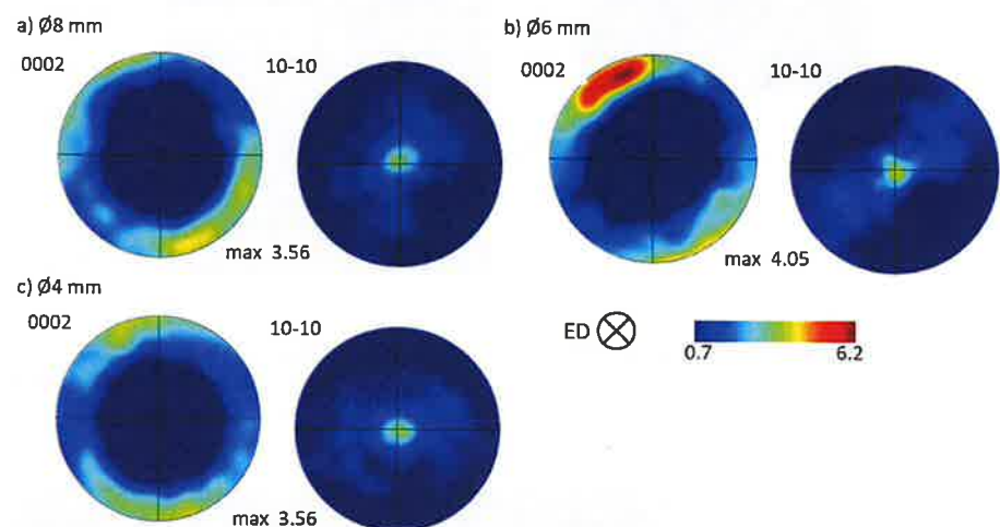
Figure 4. Pole figures (0002) and (10-10) obtained for pure Mg KoBo-extruded to a diameter of (a) Ø8 mm (R 1 5:1), (b) Ø6 mm (R 2 7:1), or (c) Ø4 mm (R 3 10:1); ED—extrusion direction.
