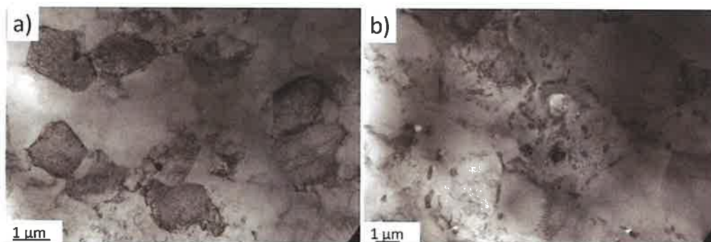
Fig. 5. TEM images of the microstructure of the alloy extruded to Ø4 mm (a), and the alloy extruded to Ø2 mm (b).
