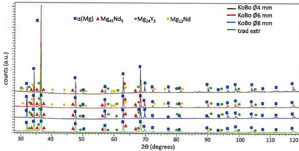
Fig. 4. Phase composition of the investigated materials analyzed with XRD.
