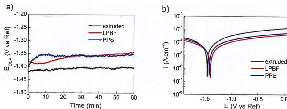
Fig. 9. Results delivered from electrochemical measurements performed in naturally aerated 0.01 M NaCl: a) E_{\text{corr}} evaluation over 1 h, b) potentiodynamic polarization curves.
