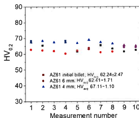
Fig. 10. Microhardness profiles of the AZ61 initial billet, AZ61 KoBo extruded to Ø6 mm and to Ø4 mm.
