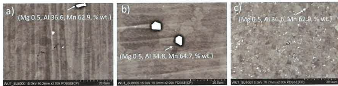
Fig. 4 – SEM microstructure images of AZ31 alloys extruded to: a) \varnothing 6 mm, b) \varnothing 4 mm, and c) \varnothing 2 mm.
