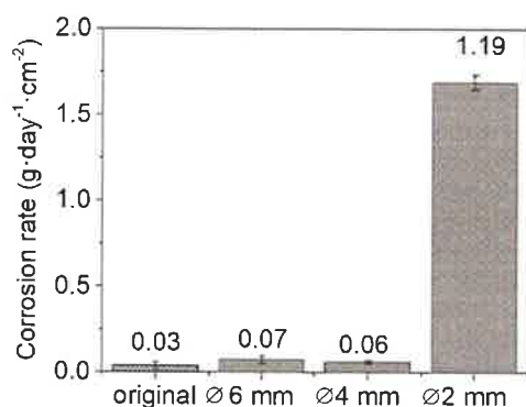
Fig. 7 – Corrosion rates calculated from mass loss measurements for the original AZ31 and the alloys extruded via KoBo to Ø6 mm, Ø4 mm, and Ø2 mm.
