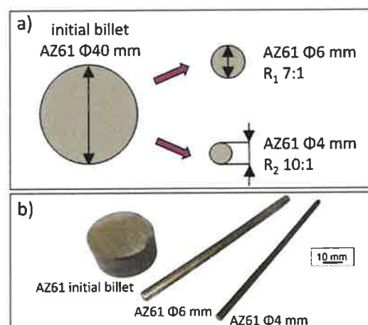
Fig. 2. Details of KoBo extrusion applied to the investigated materials: a) initial and final dimensions of the AZ61 rods extruded under various extrusion ratios, b) real life images of the extruded rods.
